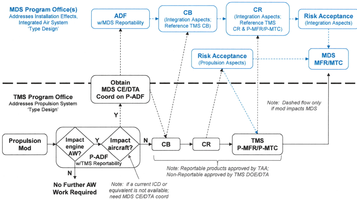
Figure 2. Propulsion System Modification Type Certification Process
